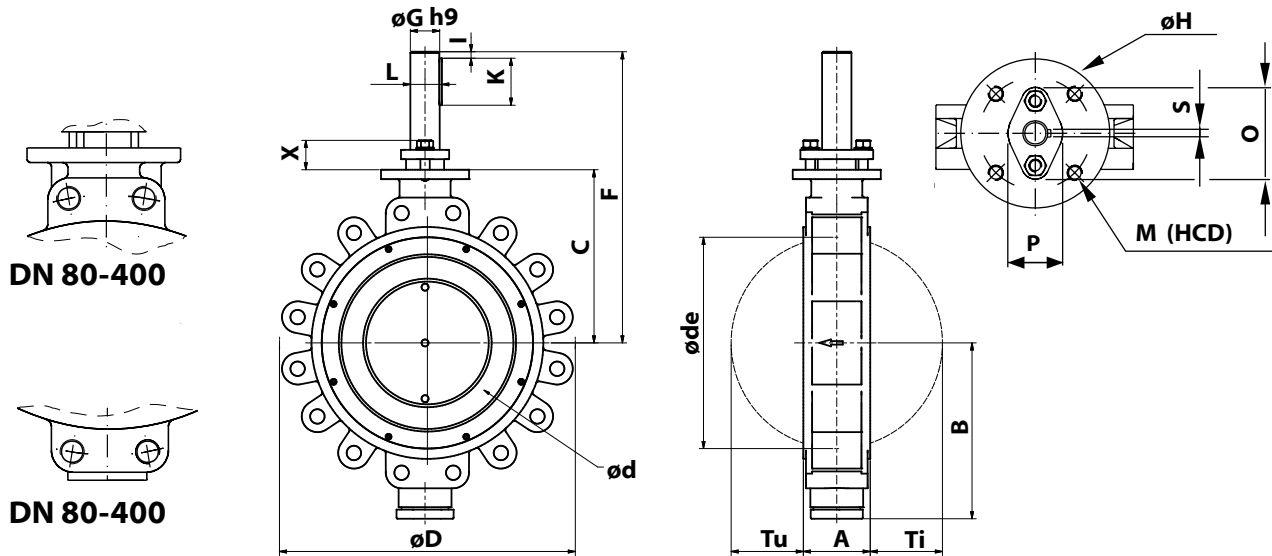
Butterfly valve type VSSL PN 40 /Class 300
