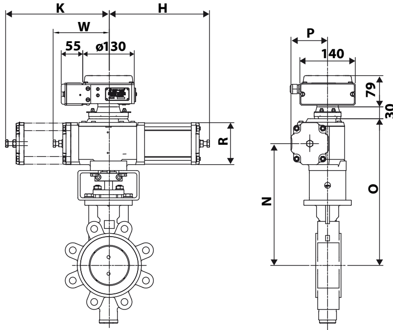
Butterfly valve type VSS PN 40/ Class 300 with actuator type A-DA
